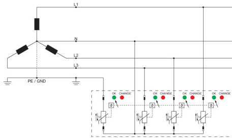
Schematic circuit diagram UL
