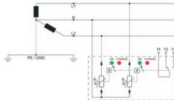
Single-phase (2 poles) Split-phase or single-phase three-wire system
