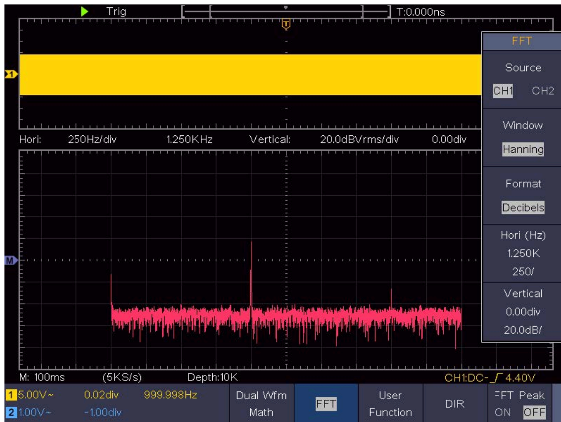
Figure 4-4 Hanning window
