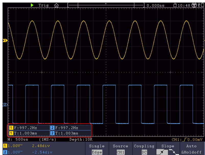
Figure 4-20 Automatic measurement
