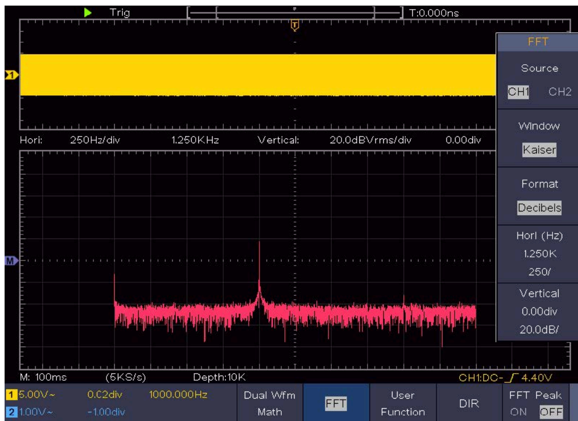
Figure 4-5 Kaiser window
