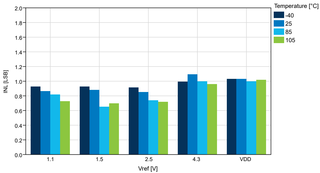
Figure 35-64. INL vs. V_{ref} ( V_{DD}=5.0\text{V} , 115ksps)
