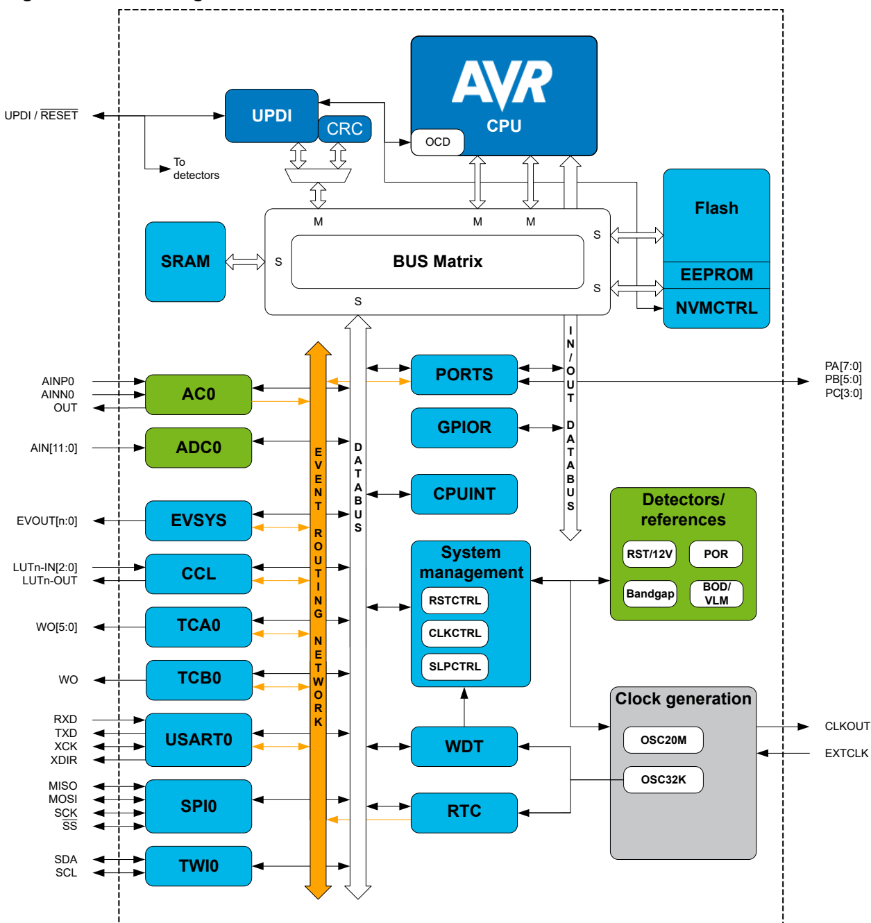
Figure 3-1. Block Diagram
