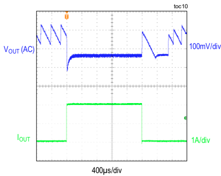
LOAD TRANSIENT ( V_{IN} = 24V, V_{OUT} = 5V, I_{OUT} = 25mA \text{ TO } 2A, \text{ PFM MODE} )
