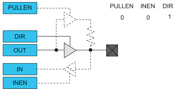
Figure 32-7. I/O Configuration - Totem-Pole Output with Enabled Input
