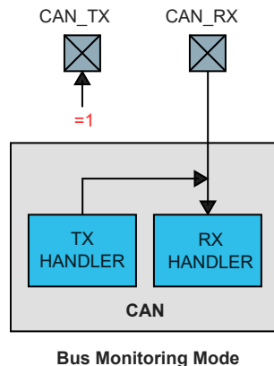
Figure 39-3. Pin Control in Bus Monitoring Mode
