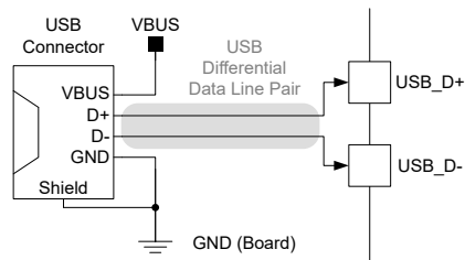
Figure 59-17. Low Cost USB Interface Example Schematic
