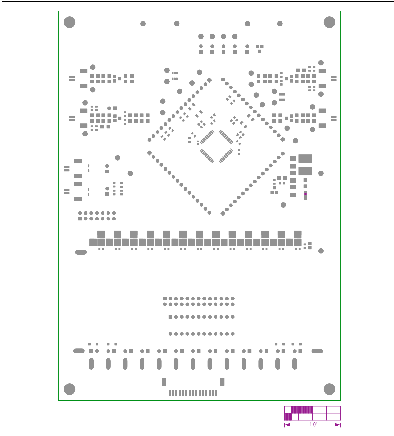
MAX17843 EV Kit PCB Layout—Top Soldermask
