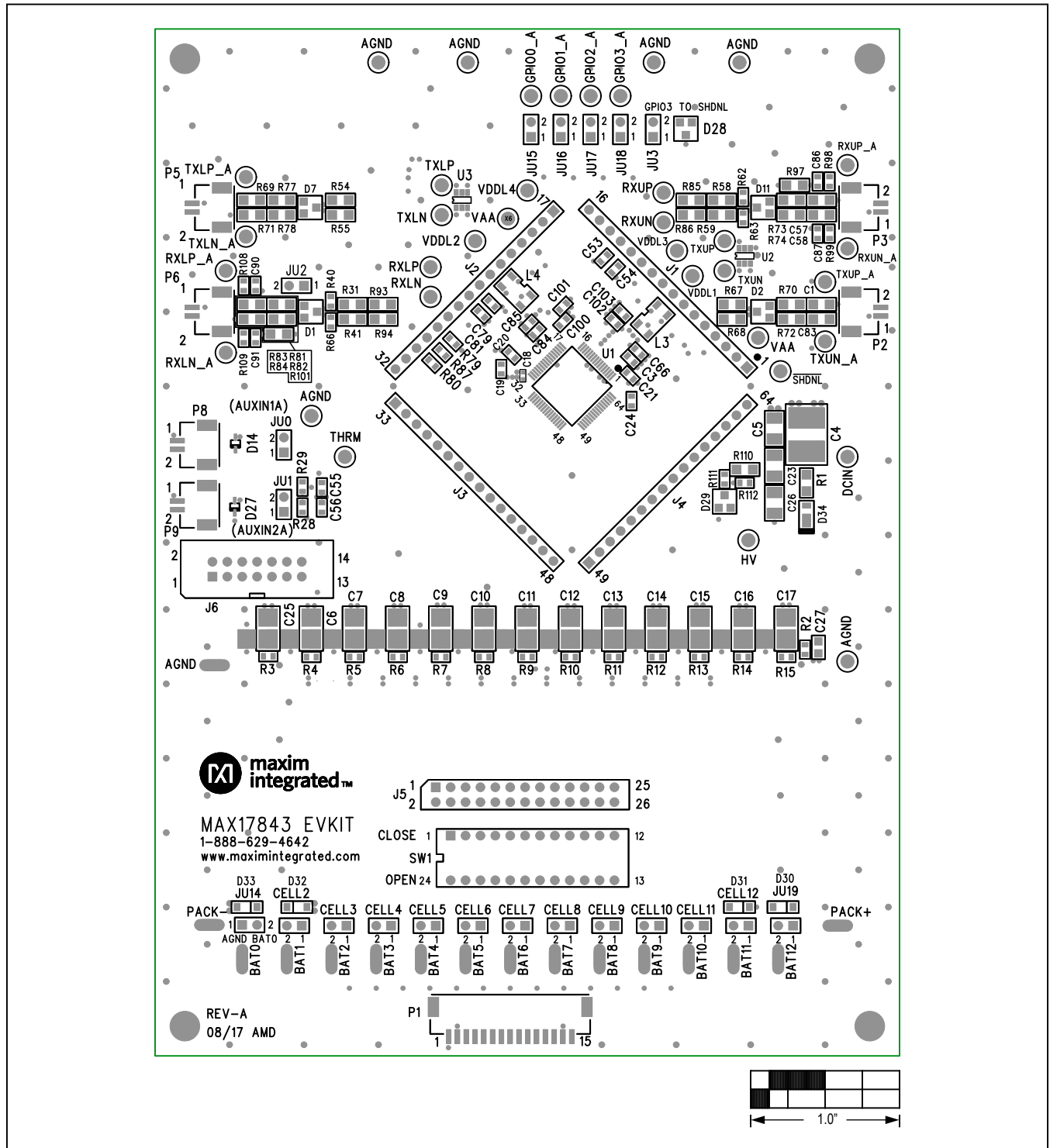
MAX17843 EV Kit Component Placement Guide—Top Silkscreen
