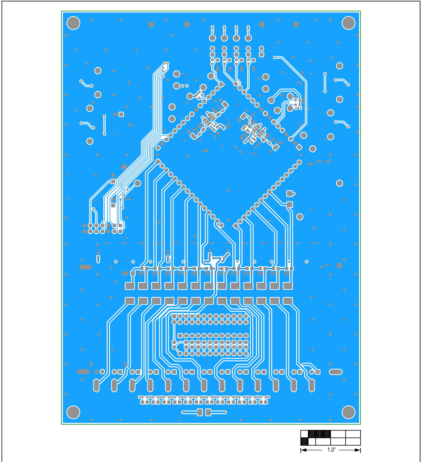
MAX17843 EV Kit PCB Layout—Solder Side
