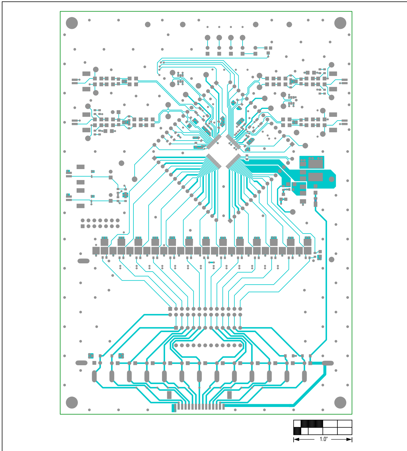
MAX17843 EV Kit PCB Layout—Component Side
