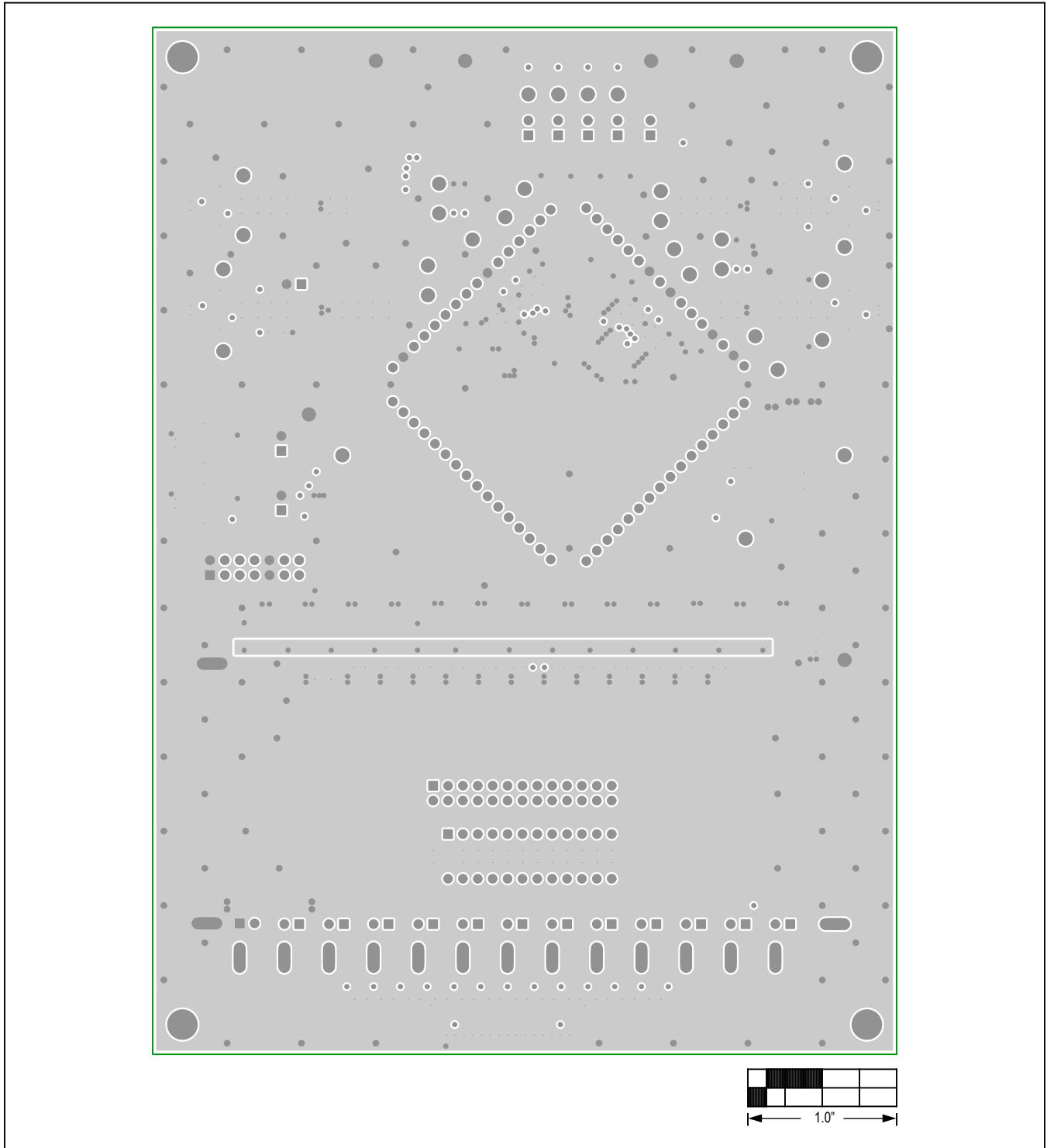
MAX17843 EV Kit PCB Layout—Layer 2 (GND)
