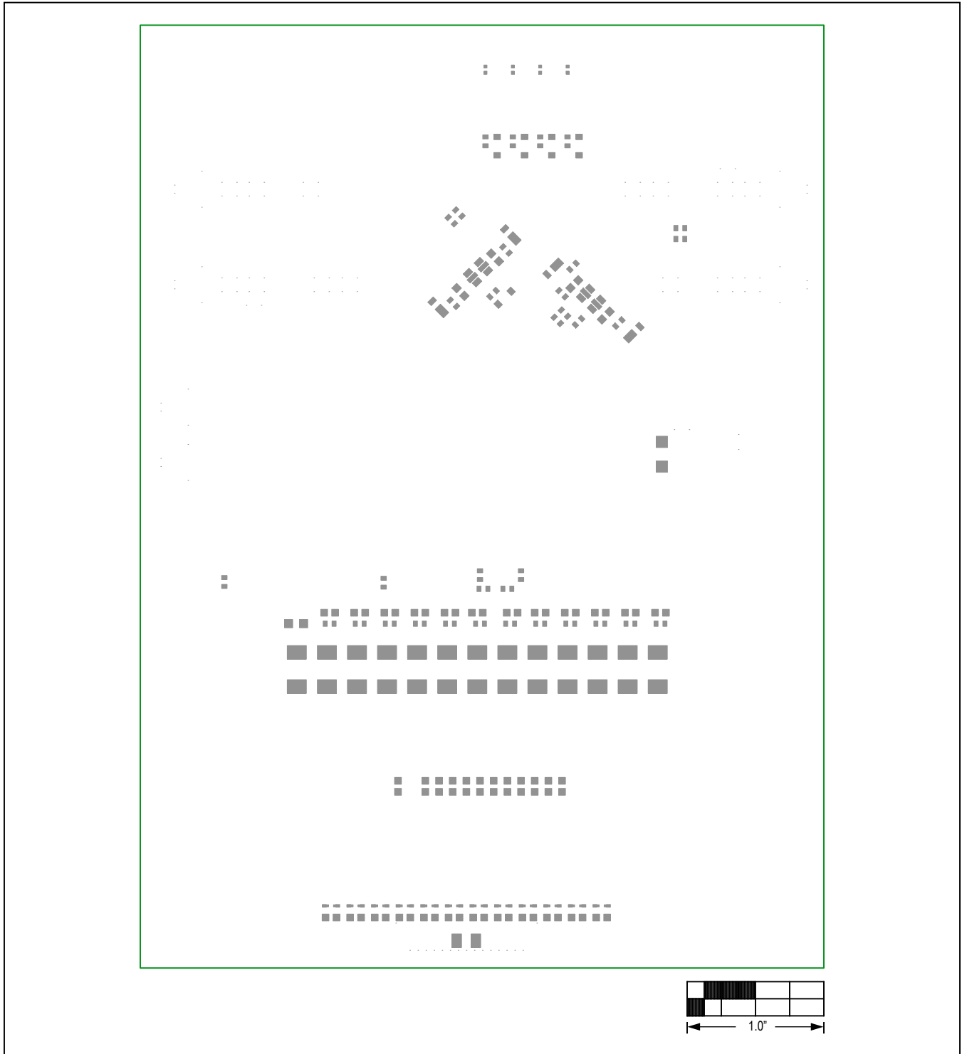
MAX17843 EV Kit PCB Layout—Bottom Pastemask
