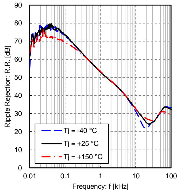
Figure 14. Ripple Rejection ( e_{in} = 1\text{ V}_{rms} , I_{OUT} = 100\text{ mA} )
