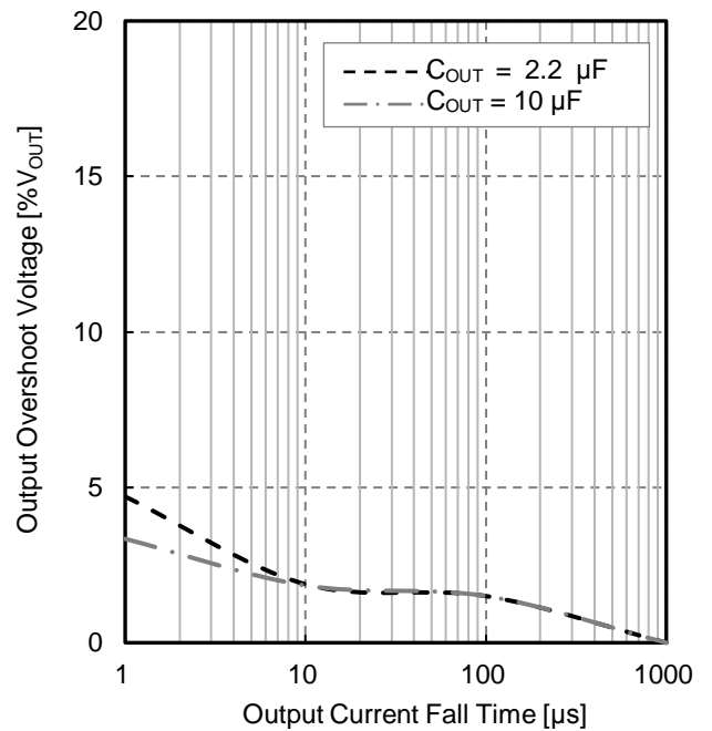
(d. I_{OUT} = 700\text{ mA} \rightarrow 1\text{ mA} , C_{ADJ} = 220\text{ pF} )
