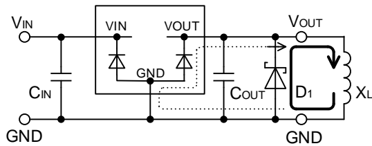
Figure 38. Current Path in Inductive Load (Output: Off)
