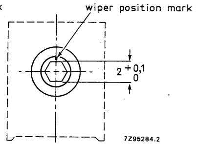
Fig. 5 Hexagonal slot, insulated wiper for vertical and horizontal versions.
