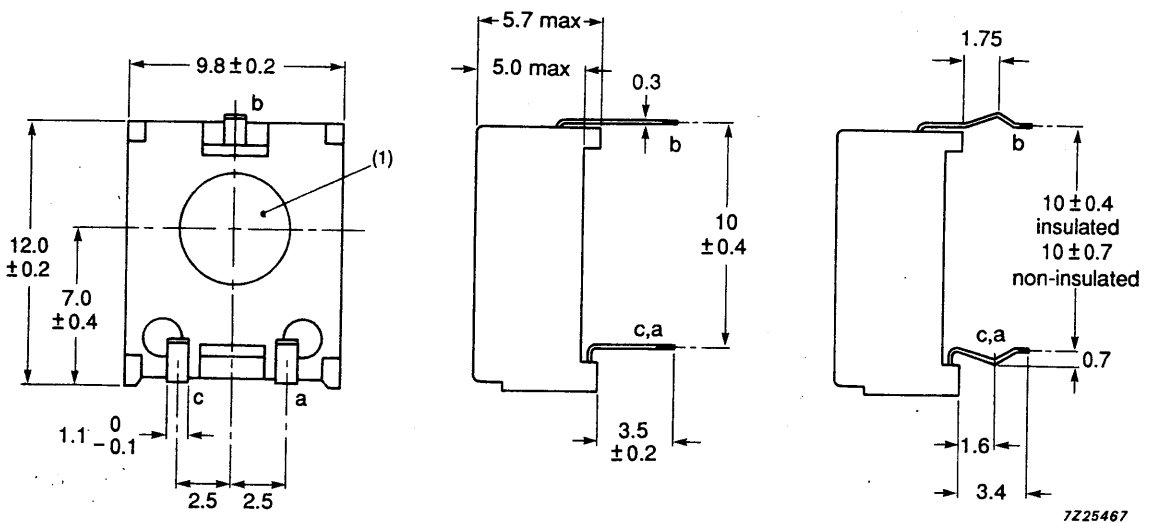
Fig. 2 Horizontal mounting.
