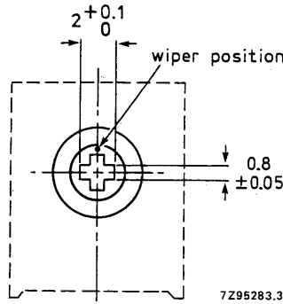
Fig. 4 Cross slot, insulated wiper for vertical and horizontal versions.
