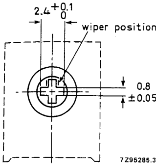
Fig. 3 Cross slot, non-insulated wiper for vertical and horizontal versions; straight pins only.
