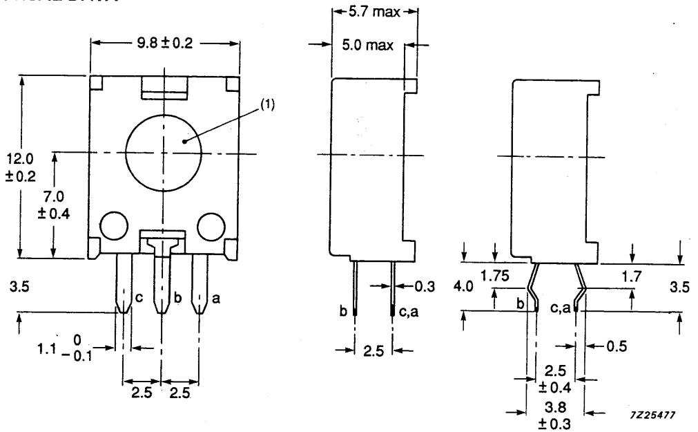
Fig. 1 Vertical mounting.
