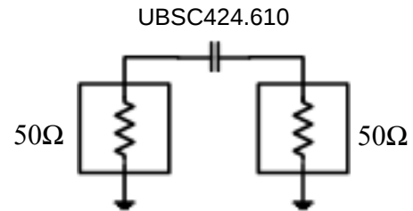
Fig.3 100nF UBSC measurement schematic
