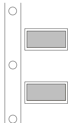
Fig. 13: Die orientation (flip) within the carrier (Pocket) related to tape and reel orientation
