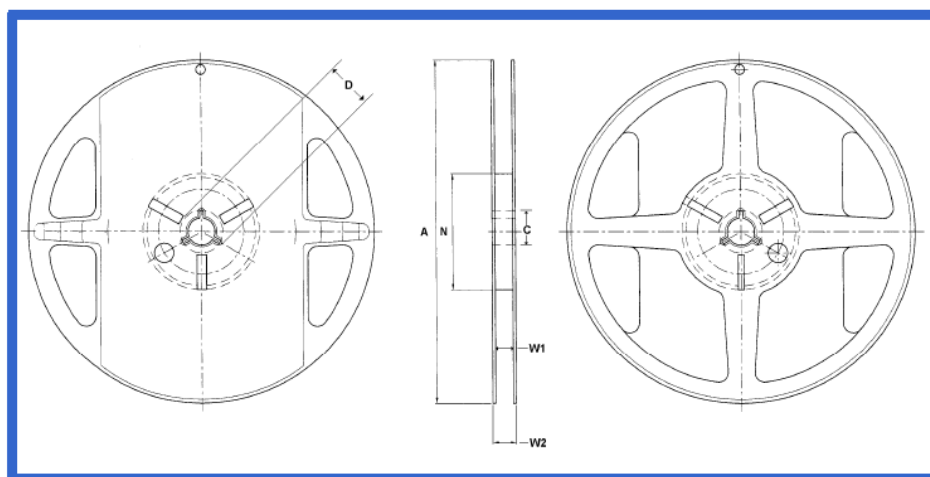
Fig. 14 : Reel references and dimensions used for tape width 8mm
