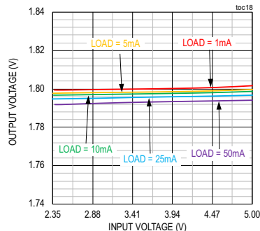
MAX17672C, 1.8V OUTPUT LINEAR REGULATOR, OUTPUT VOLTAGE vs. INPUT VOLTAGE
