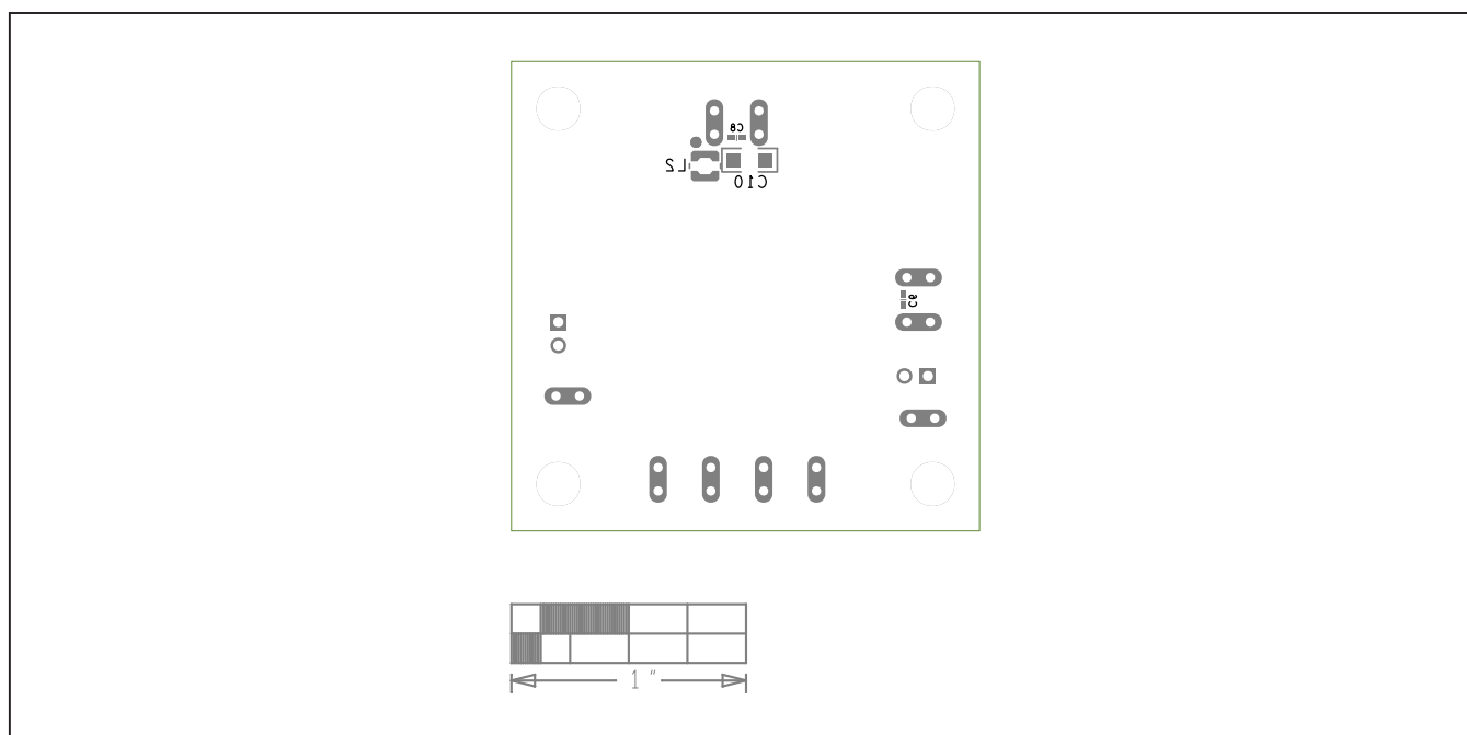
MAX17672C EV Kit—Bottom Silkscreen
