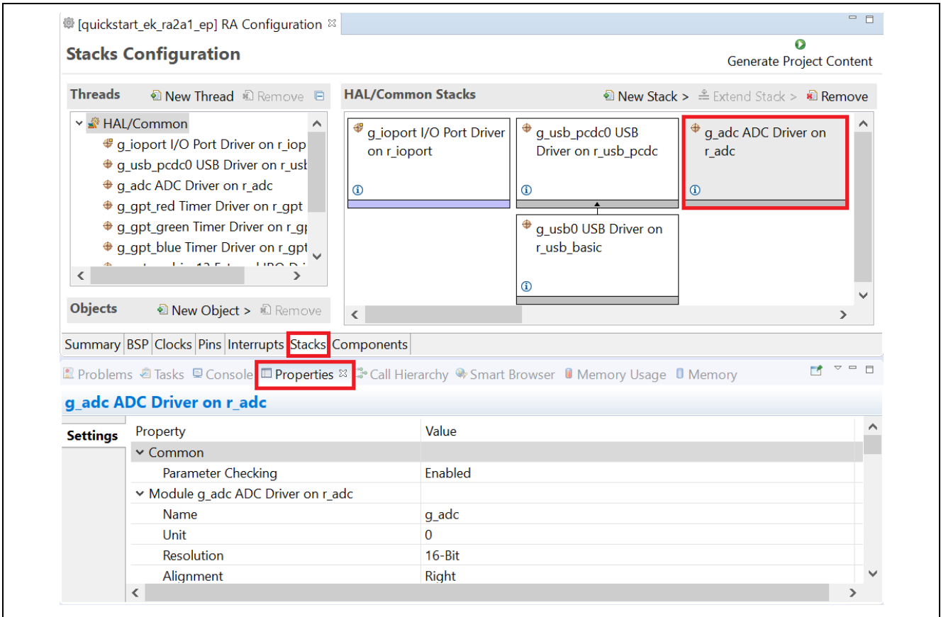
Figure 17. Modifying the Configuration Settings
