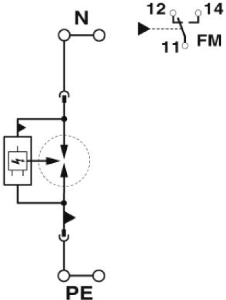
Circuit diagram
