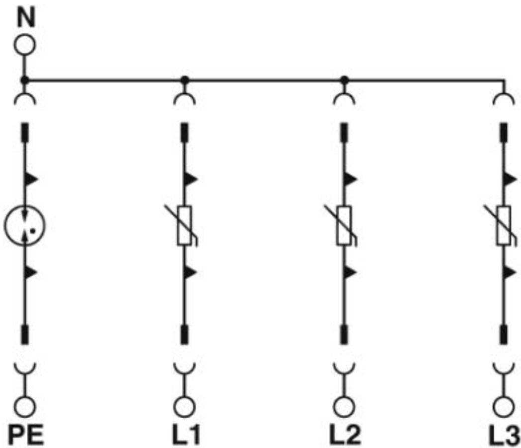
Circuit diagram
