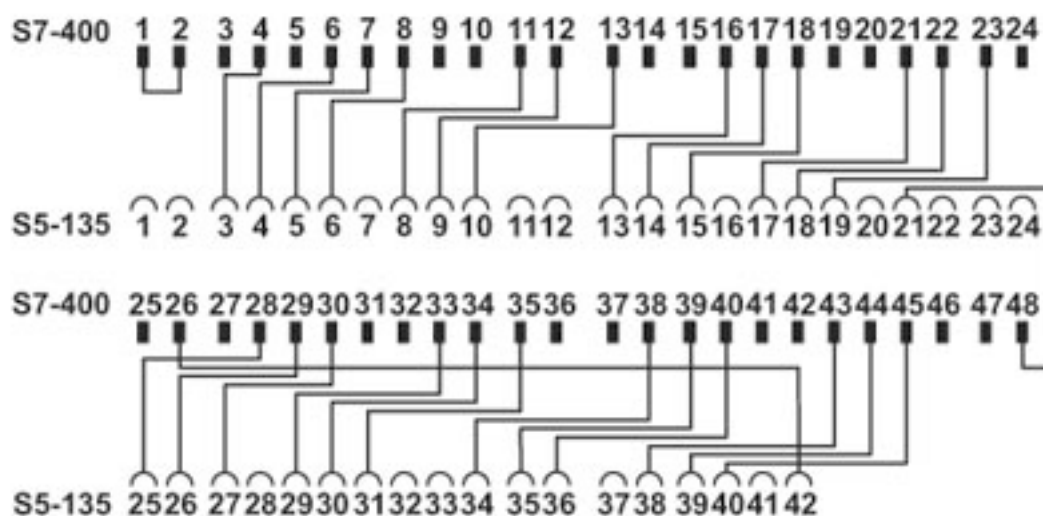
Connection scheme FLKM S135-470-4UC/U/S400
