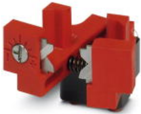
Adjustable spare stripping knife, 1.0 mm 2 , for crimping machine CF 3000
