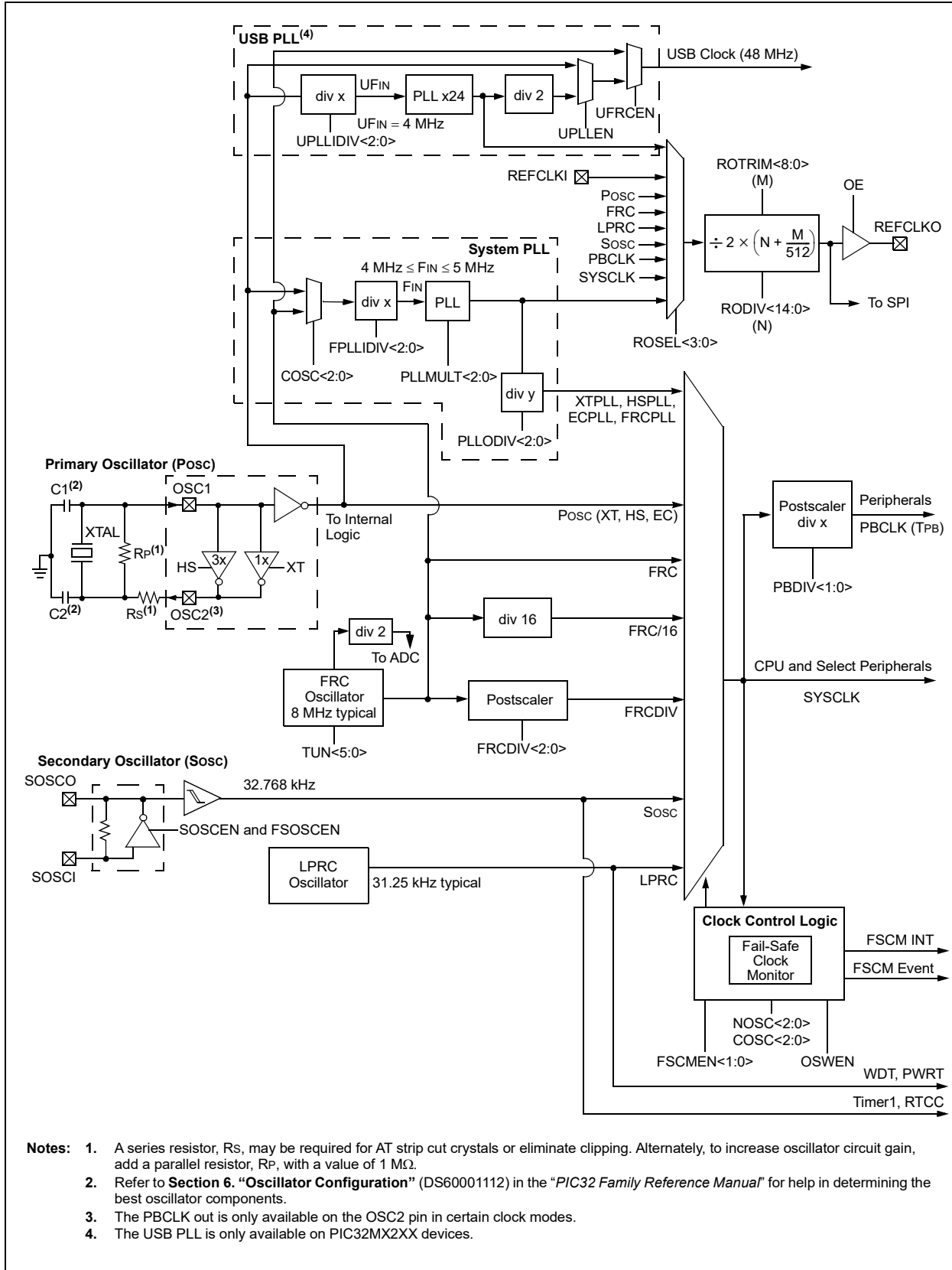
FIGURE 8-1: OSCILLATOR DIAGRAM
