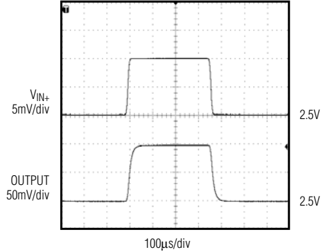
LARGE-SIGNAL PULSE RESPONSE TIME MAX4208/9 ttc17
