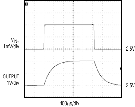
LARGE-SIGNAL PULSE RESPONSE TIME MAX4208/9 ttc19
