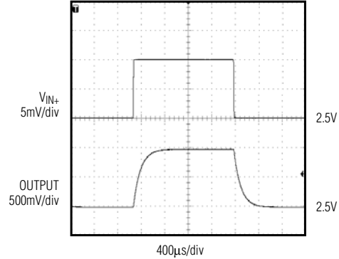
LARGE-SIGNAL PULSE RESPONSE TIME MAX4208/9 ttc18
