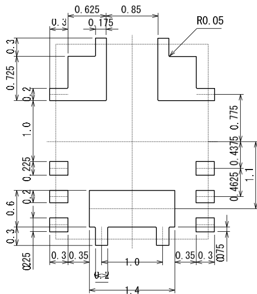
● Reference Metal Mask Design (unit: mm)
