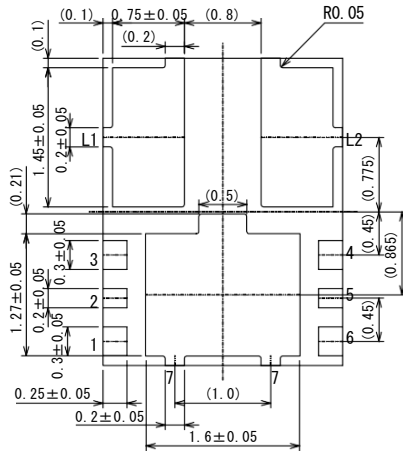
● Reference Pattern Layout (unit: mm)
