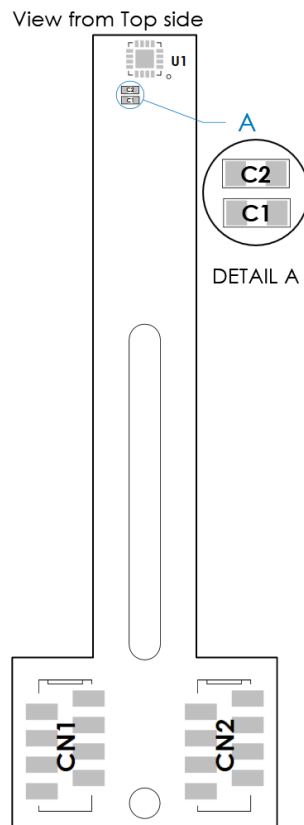
Figure 16: Assembly View LT Type 2
