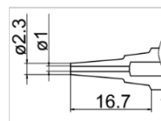
N3-L10 Nozzle Size Φ1.0(Long)
