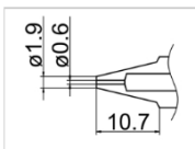
N3-06 Nozzle Size Φ0.6
