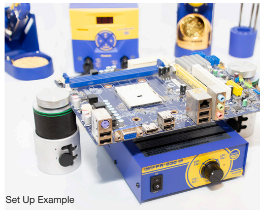
C5028 Rework Fixture
