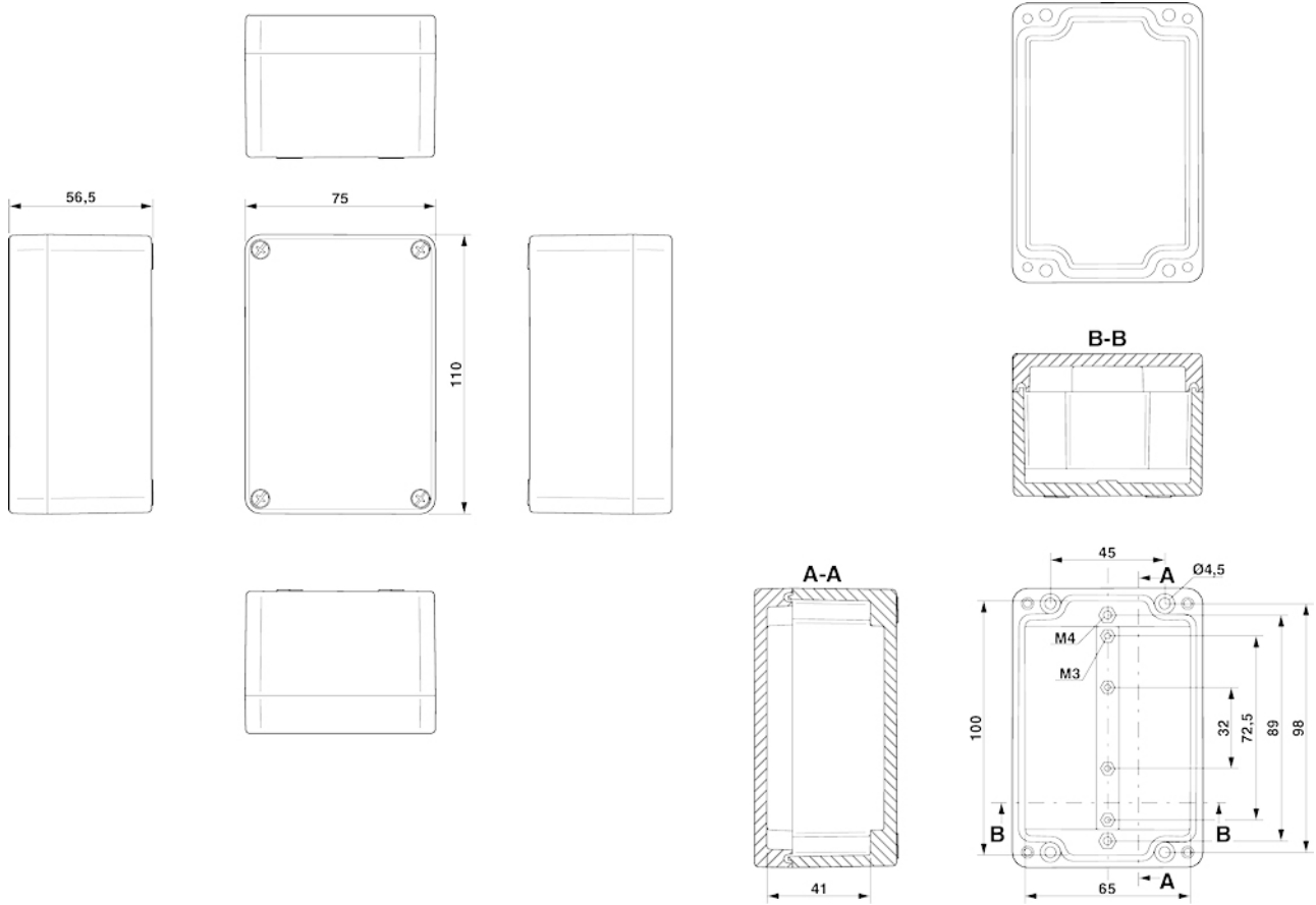
Dimensional drawing
