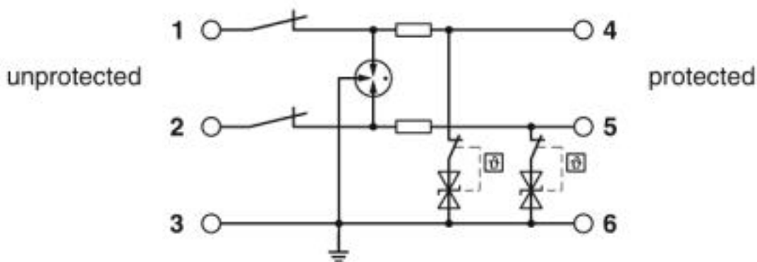
Circuit diagram
