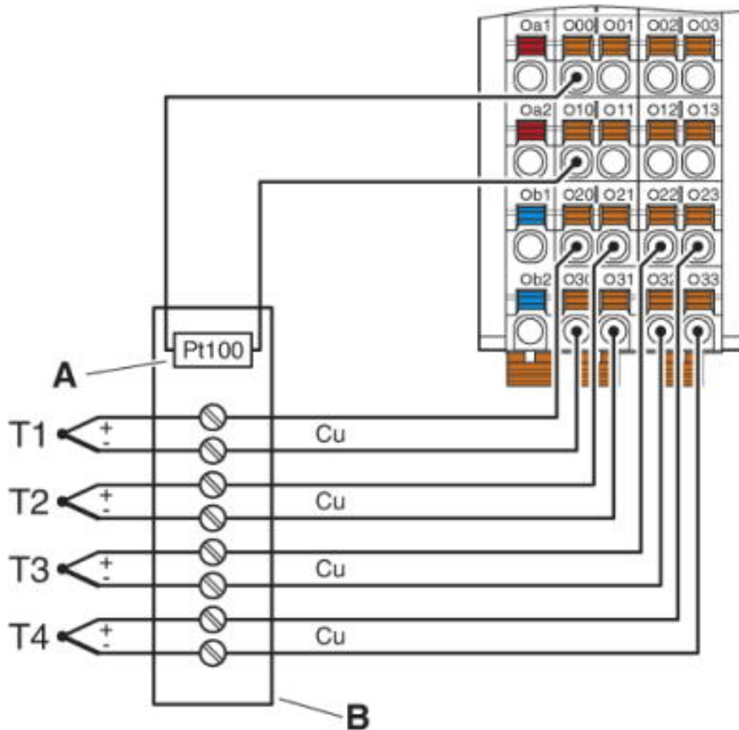
Connection diagram
