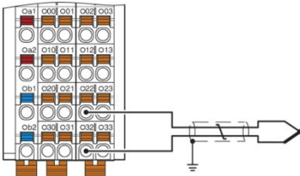
Connection diagram
