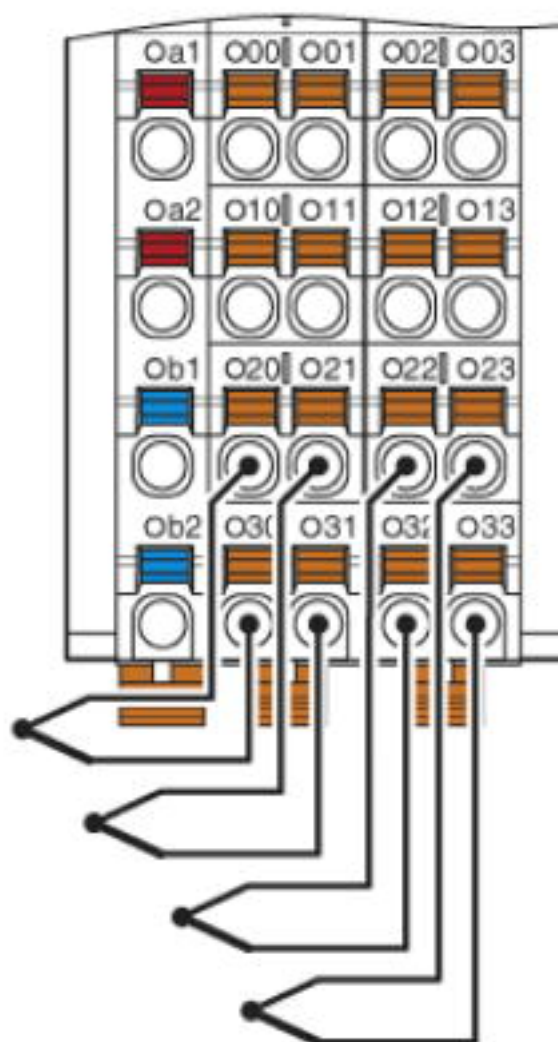
Connection diagram
