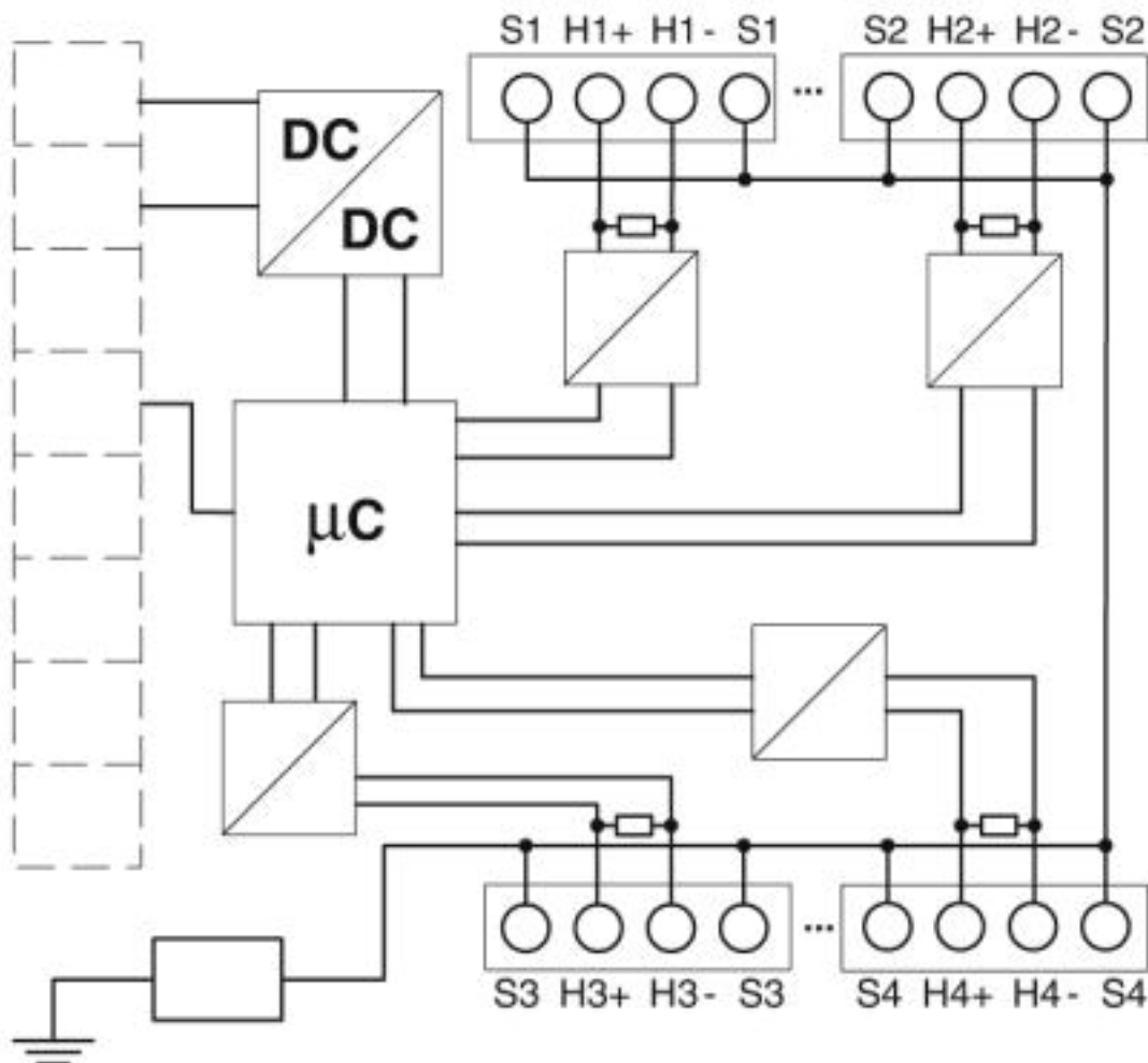
Block diagram
