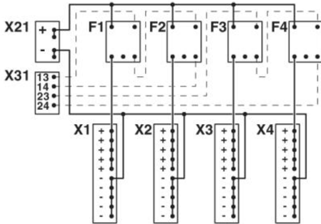
Circuit diagram
