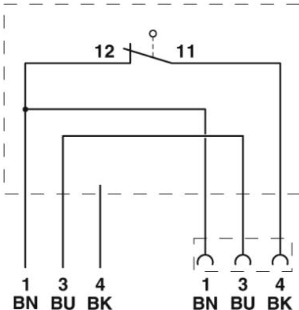
Circuit diagram
