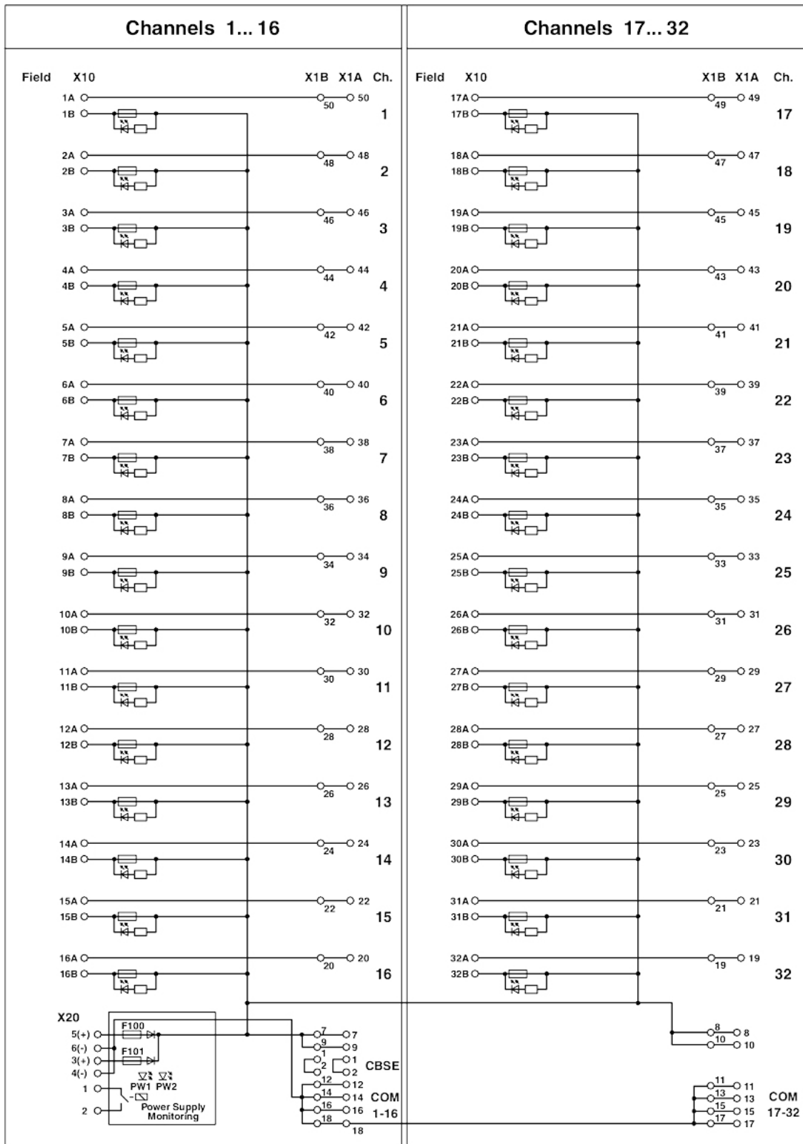
Circuit diagram
