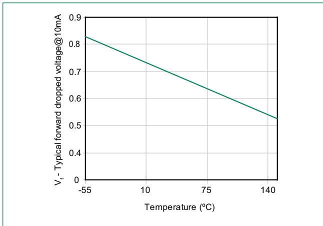
Figure 5 - Forward Voltage
