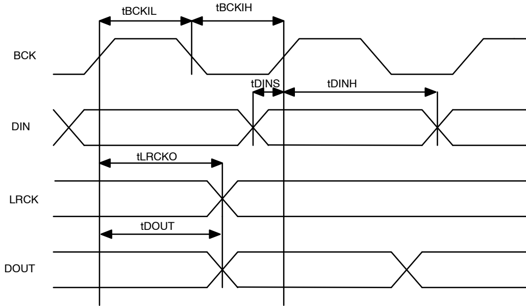
Figure 16. Master Mode
