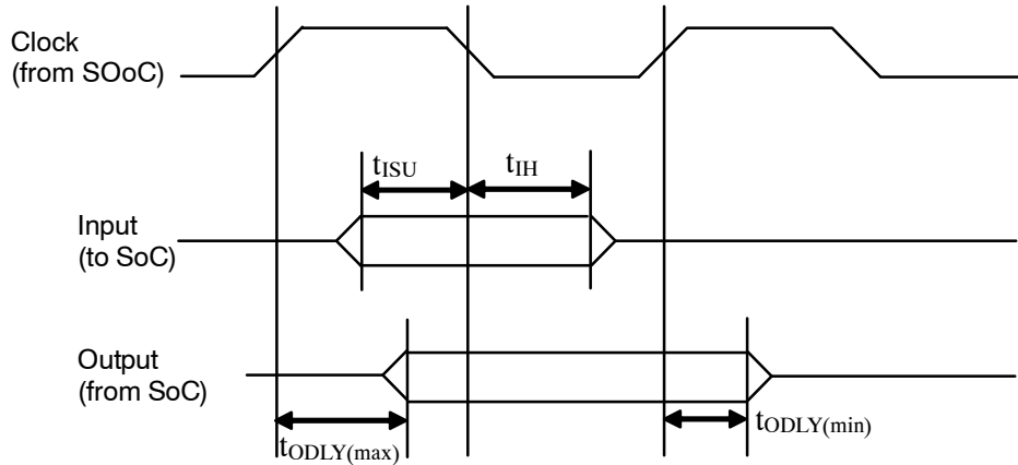
Figure 15. AC Characteristics – PSRAM Interface
