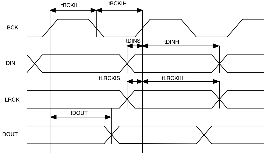
Figure 17. Slave Mode
