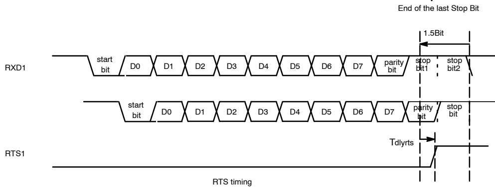
Figure 28. RTS Timing
