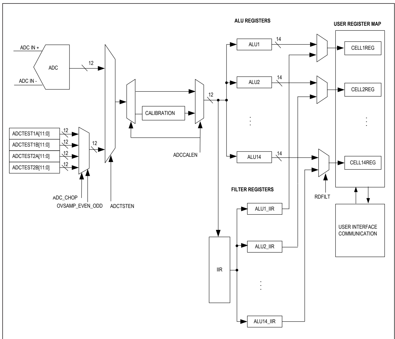
Figure 34. Data-Flow Diagram
