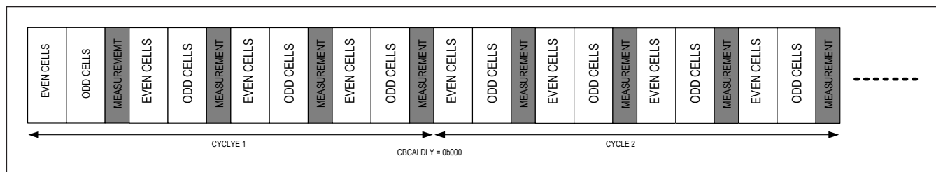
Figure 46. Cell Balancing with No Calibration
