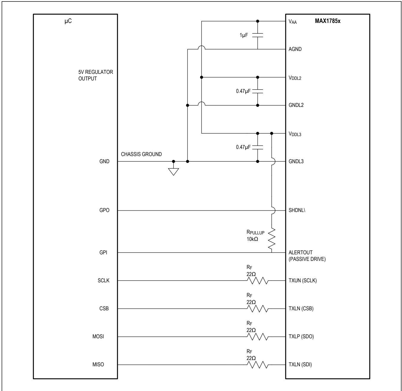
Figure 110. 3.3V SPI Supply from Device V_{AA} LDO
