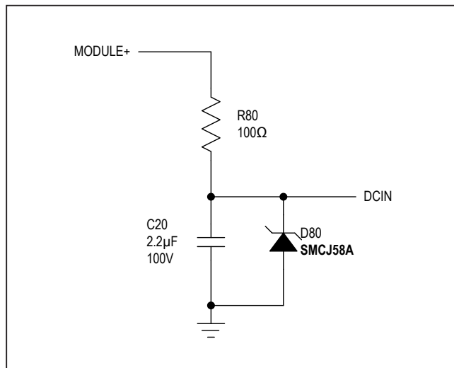
Figure 99. Power-Supply Connection
