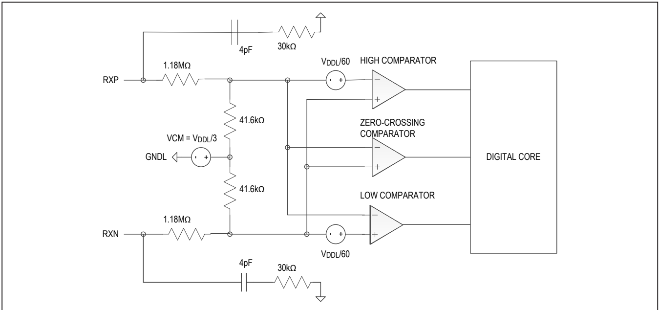
Figure 58. UART Receiver
