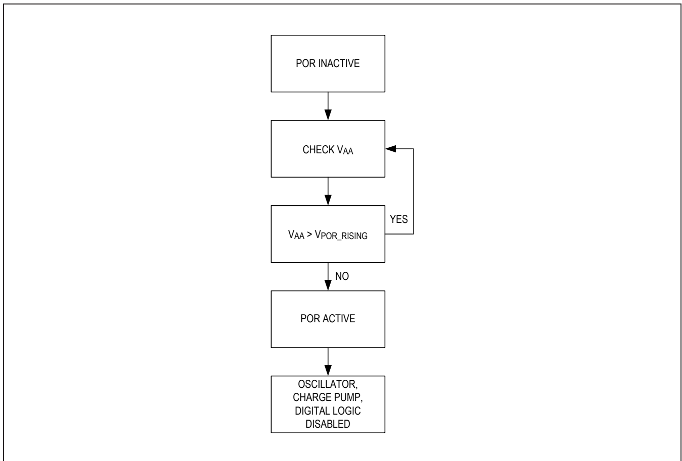
Figure 13. Shutdown Sequence
