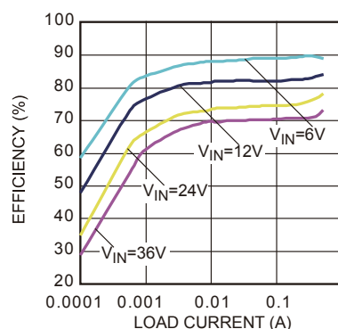
Efficiency vs. Load Current V_{OUT}=3.3V
