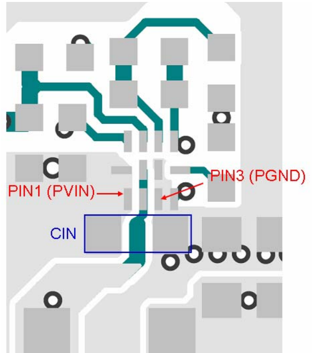
Figure 5—Two Ends off Input Decoupling Capacitor Close to Pin 1 and Pin 3
