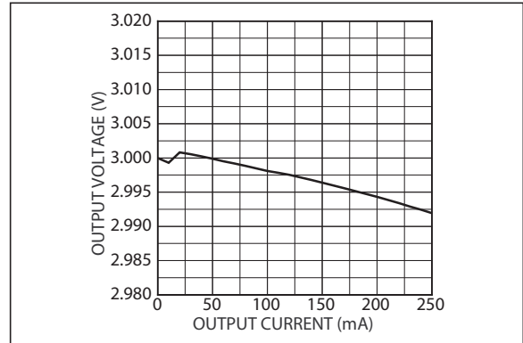
FIGURE 2-18: Load Regulation LDO 2.
