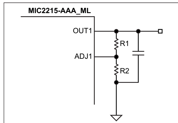
FIGURE 5-1: Adjustable Output.
