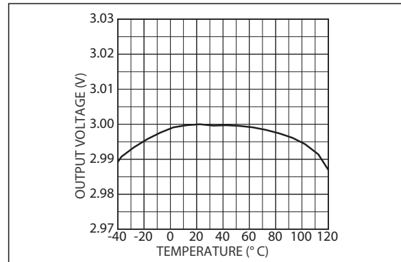
FIGURE 2-5: Output Voltage vs. Temperature for LDO 2.
