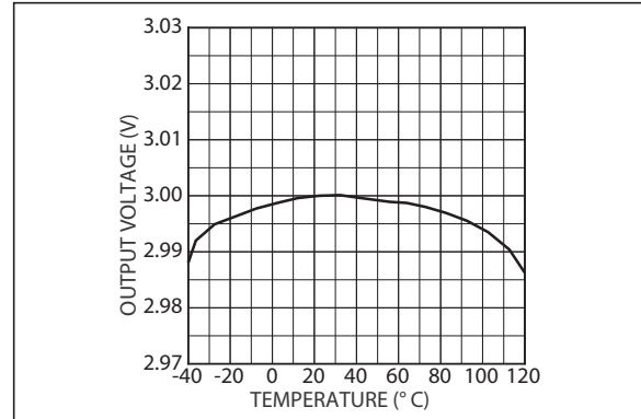
FIGURE 2-4: Output Voltage vs. Temperature for LDO 1.
