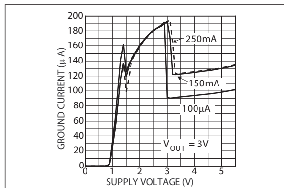
FIGURE 2-24: Ground Current vs. Supply Voltage for LDO 2.
