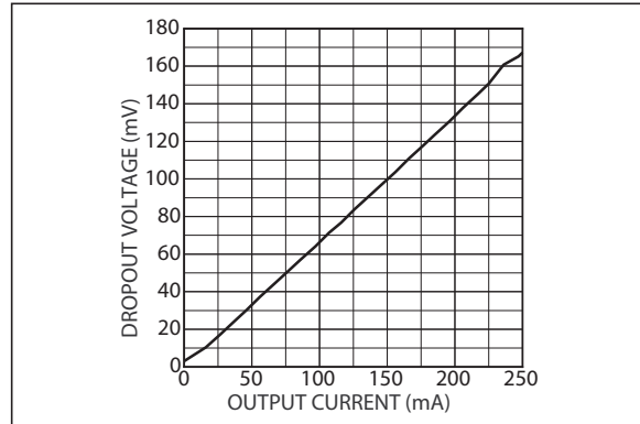
FIGURE 2-22: Dropout Voltage vs. Output Current for LDO 3.
