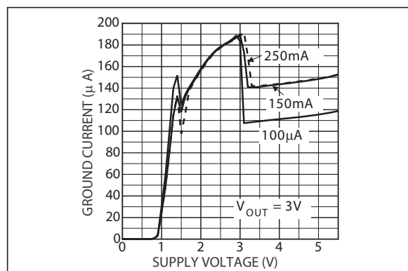
FIGURE 2-23: Ground Current vs. Supply Voltage for LDO 1.
