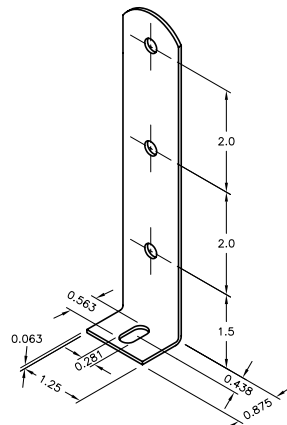
Brackets Dimensions
