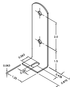
Brackets Dimensions
