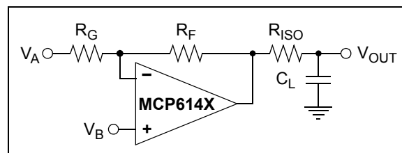
FIGURE 4-6: Output Resistor, R_{ISO} stabilizes large capacitive loads.
