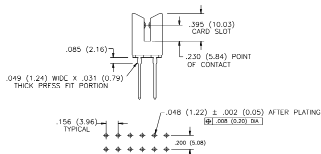
RECOMMENDED HOLE PATTERN FOR PRESS FIT
