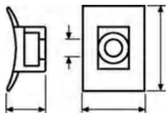
Cable Tie Mounts LKC Series
