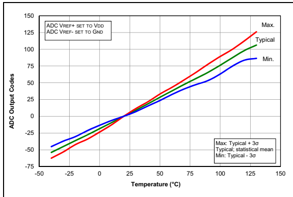
FIGURE 38-91: Temperature Indicator Slope Normalized to 20^\circ C , Low Range, V_{DD} = 3.0V , PIC16F1777/8/9 only.
