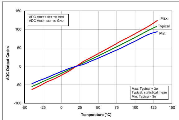
FIGURE 38-93: Temp. Indicator Slope Normalized to 20^\circ C , Low Range, V_{DD} = 3.0V , PIC16LF1777/8/9 Only.
