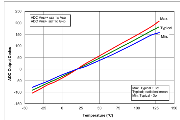
FIGURE 38-94: Temp. Indicator Slope Normalized to 20^\circ C , High Range, V_{DD} = 3.6V , PIC16LF1777/8/9 Only.
