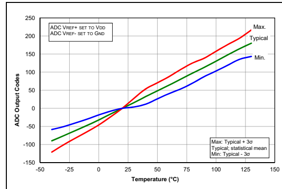
FIGURE 38-92: Temp. Indicator Slope Normalized to 20^\circ C , Low Range, V_{DD} = 1.8V , PIC16LF1777/8/9 Only.
