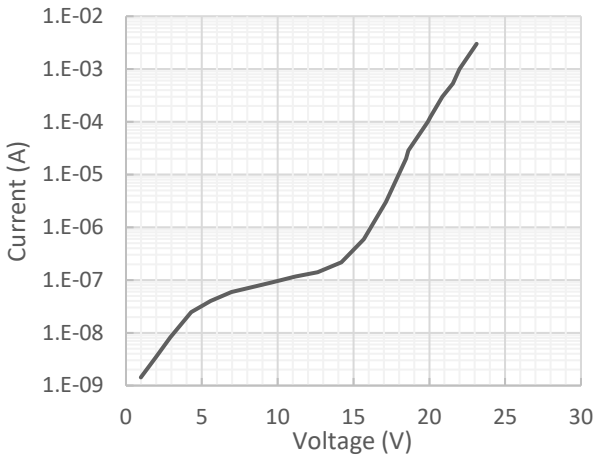
Current - Voltage
