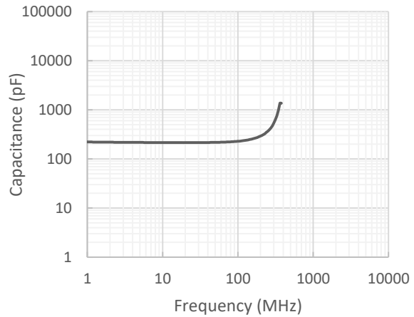
Capacitance - Freq.
