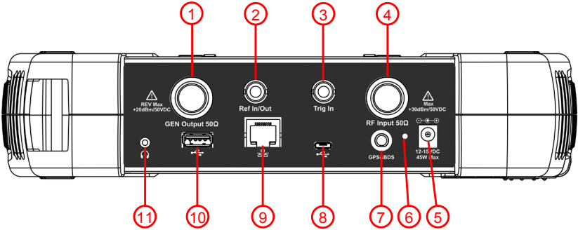
Figure 4-2 Top panel
