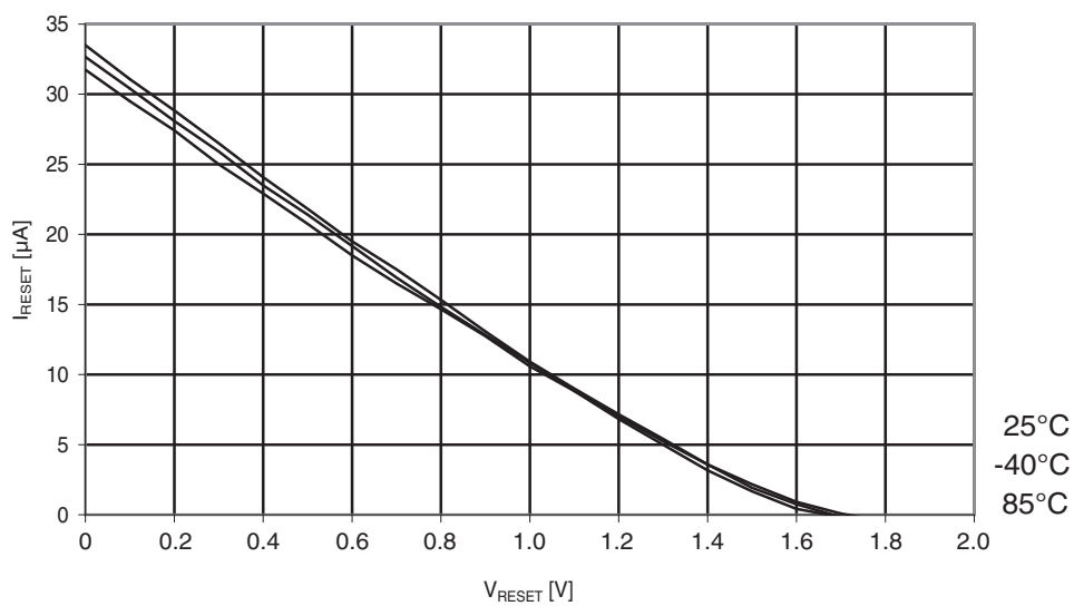
Figure 30-214. ATmega644A: Reset pull-up resistor current vs. reset pin voltage ( V_{CC} = 1.8V )
