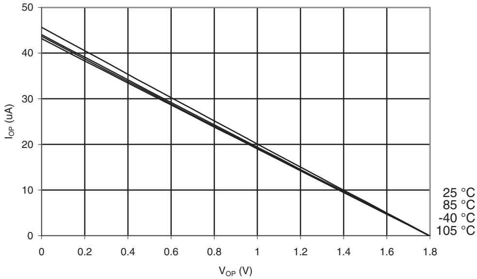
Figure 31-89. I/O Pin Pull-up Resistor Current vs. Input Voltage ( V_{CC} = 1.8V )
