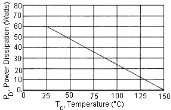
Power Derating
