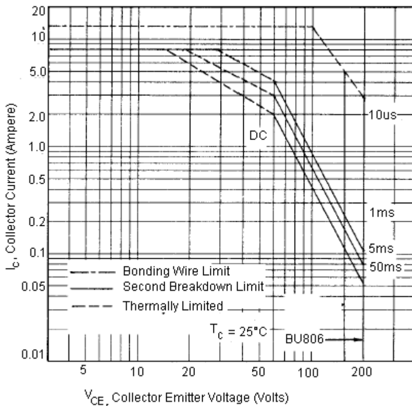
Figure 3 Active Region Safe Operating Area
