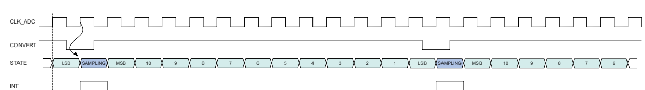
Figure 42-6. ADC Timing for Free Running in 12-bit Resolution
