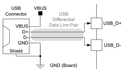
Figure 50-16. Low Cost USB Interface Example Schematic
