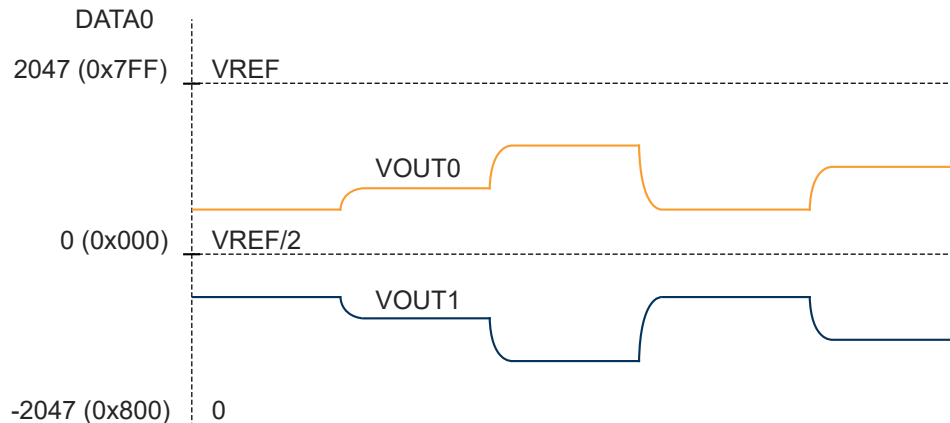
Figure 44-4. DAC Conversions in Differential Mode
