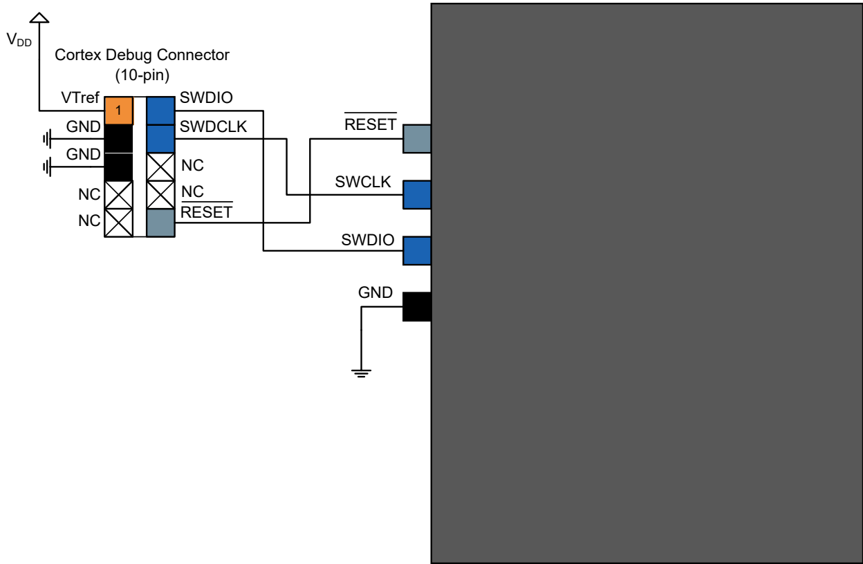
Figure 50-13. Cortex Debug Connector (10-pin)
