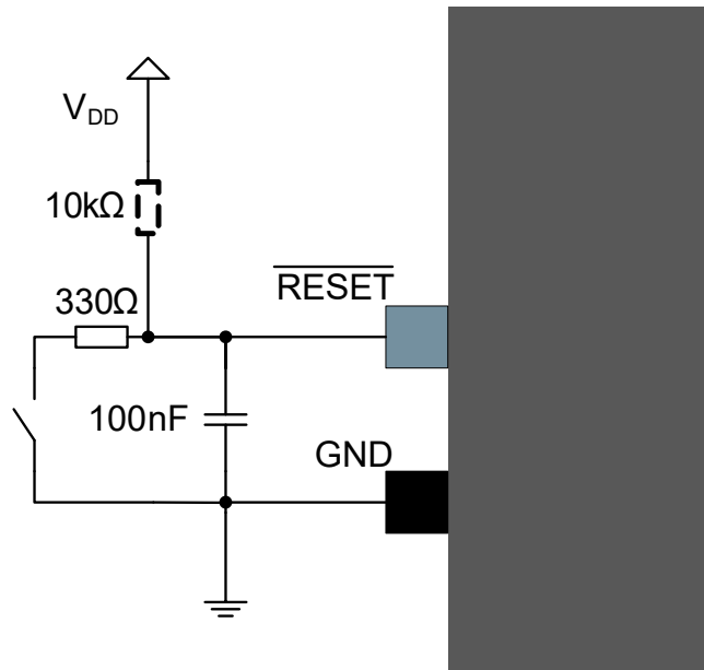
Figure 50-7. External Reset Circuit Schematic (EFT Immunity Enhancement)
