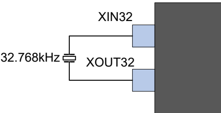
Figure 50-10. External Real Time Oscillator without Load Capacitor
