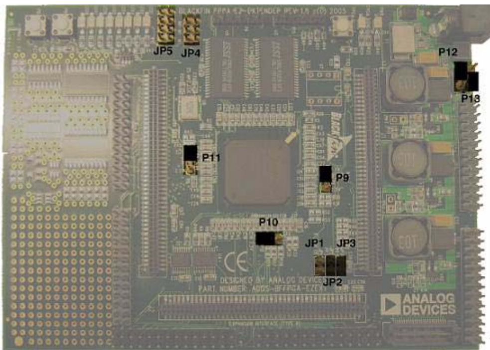
Figure 2-3. Jumper Locations
