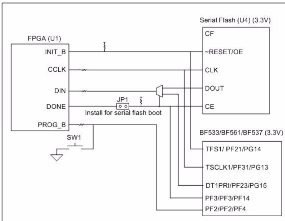
Figure 2-2. FPGA Programming Block Diagram
