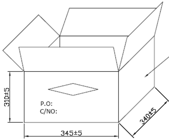
PK Carton box:A=B
